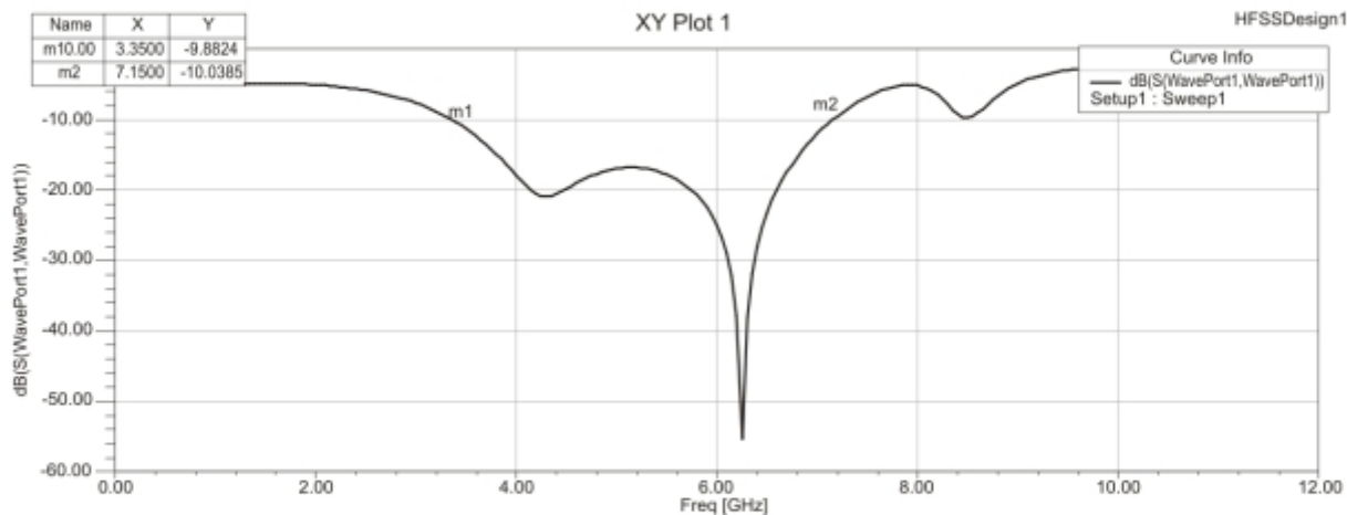
Figure 2: Return loss Vs frequency Graph
